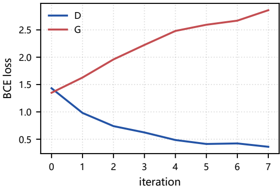
DCGAN 损失
