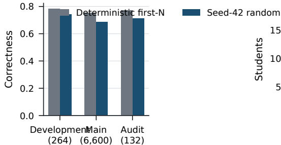
Correctness mean
