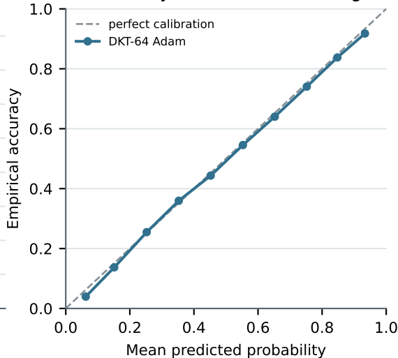
Reliability curve (clean training)
