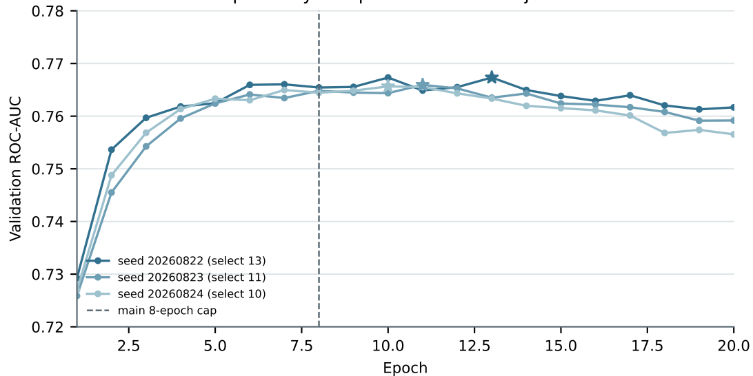
Exploratory 20-epoch validation trajectories
