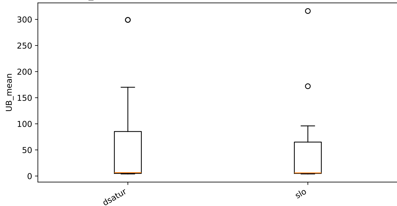
UB_mean distribution across instances (ablation=baseline)
