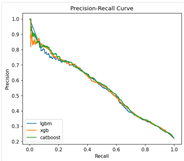
Precision-Recall Curve
