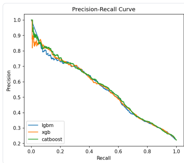
Precision-Recall Curve
