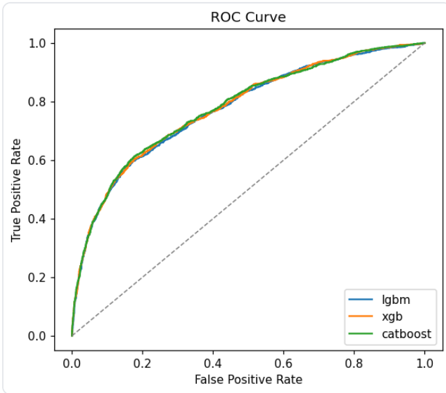
ROC Curve
