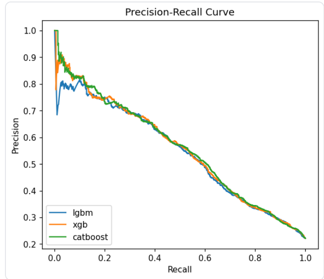
Precision-Recall Curve
