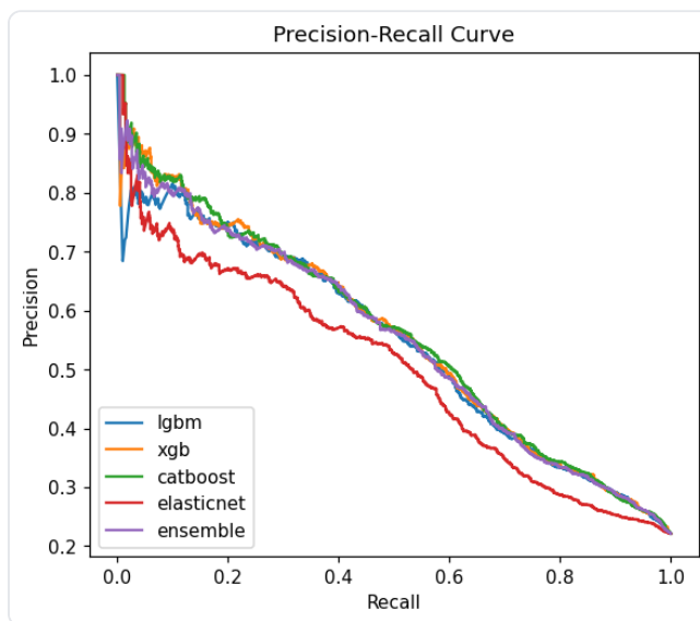
Precision-Recall Curve
