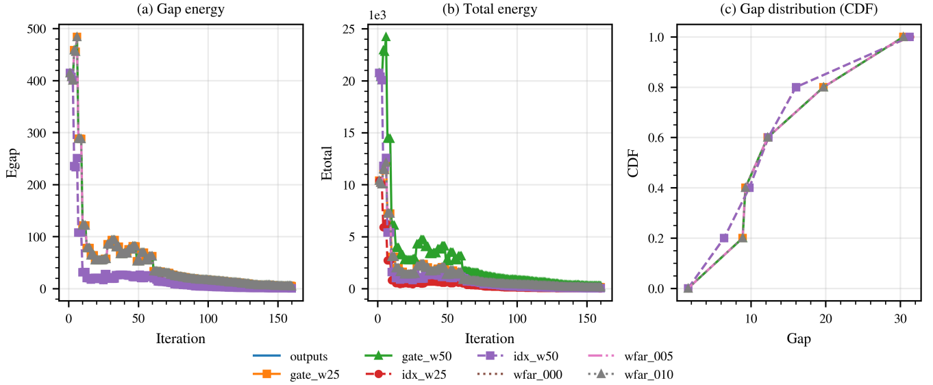
FIGURE 10. Optimization behavior and contact statistics for the impeller case (current artifact, fixed evaluation scale). (a) Gap energy E_{\text{gap}} over iterations. (b) Total energy E_{\text{total}} over iterations. (c) Empirical CDF of edge-wise gaps at convergence for all configurations (baseline, GATE_W25, GATE_W50, IDX_W25, IDX_W50, and wfar schedule variants).
