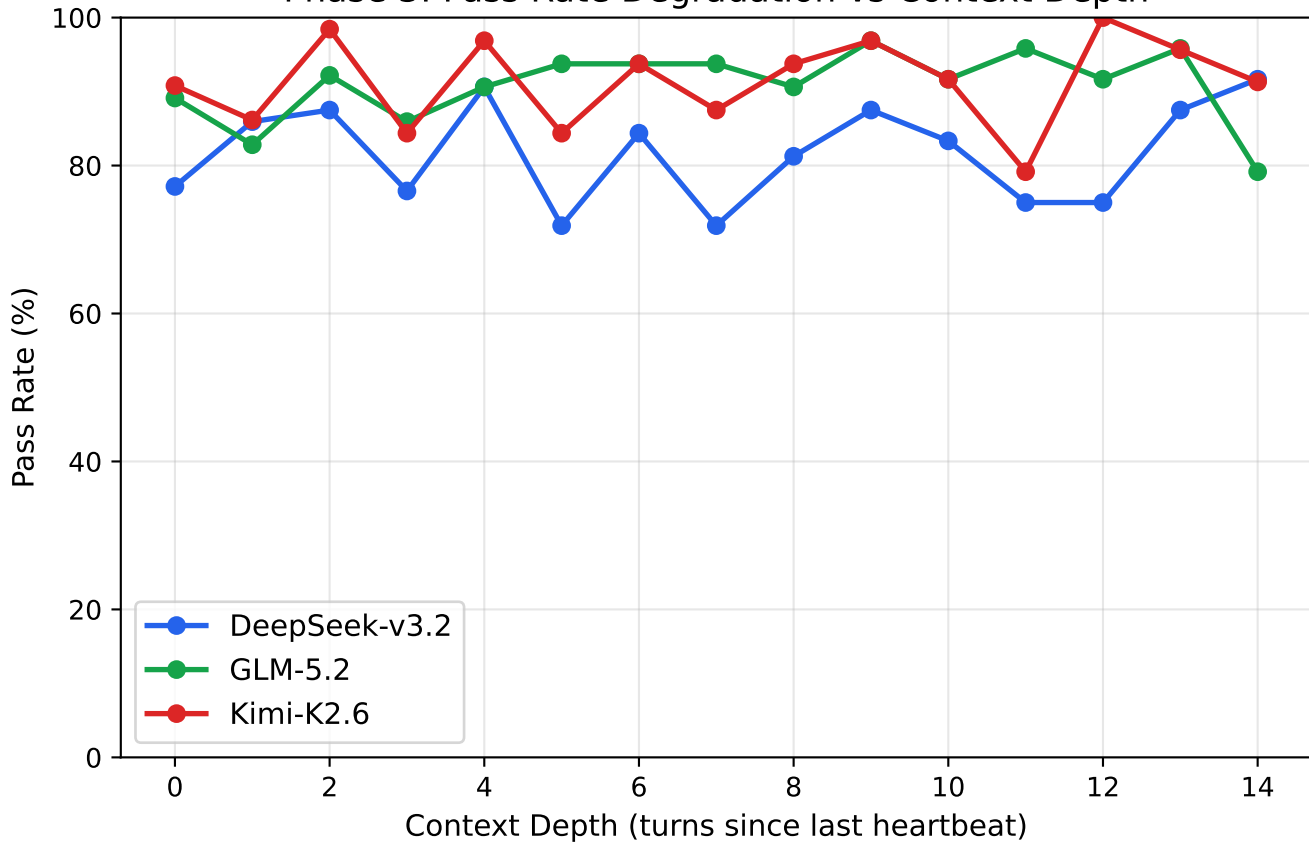
Phase 3: Pass Rate Degradation vs Context Depth
