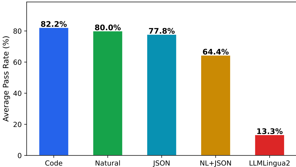
Phase 2: Frontend Average Pass Rate (across 5 models)
