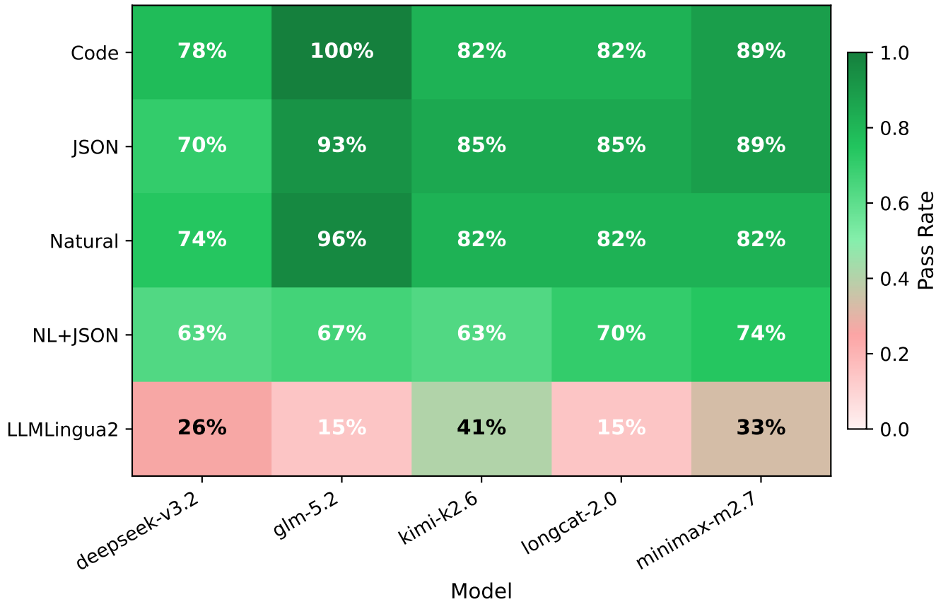
Phase 2: Pass-Rate Matrix (Frontend × Model)
