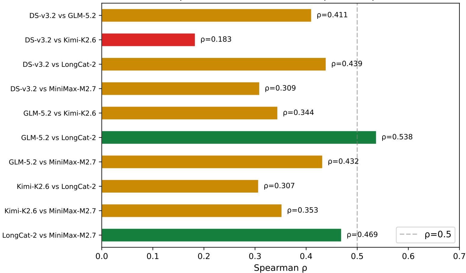
Phase 2: Pairwise Spearman Rank Correlation (per-case-per-frontend, n=135)
