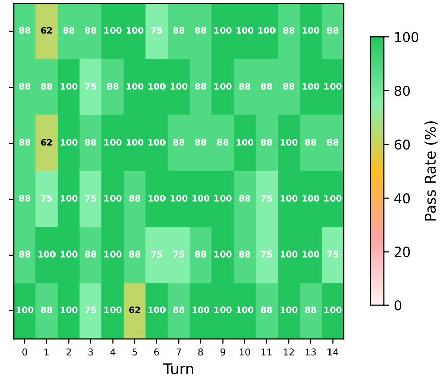
Kimi-K2.6
