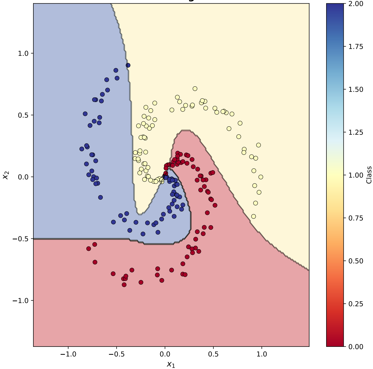
Decision Regions
