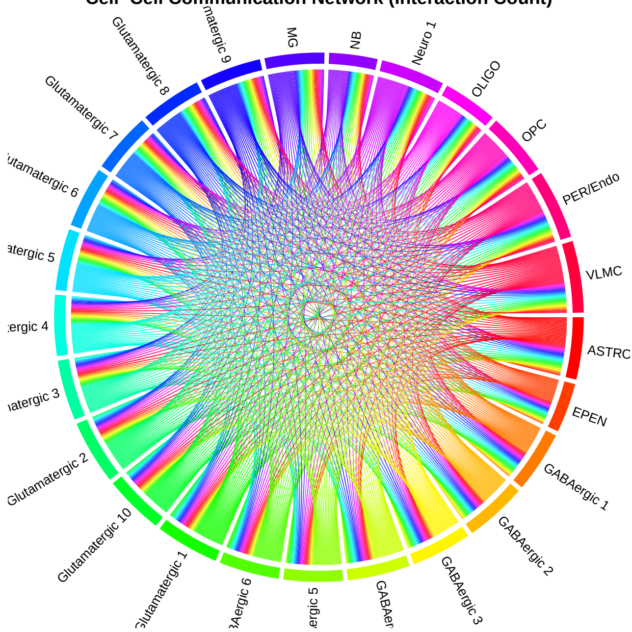
Cell-Cell Communication Network (Interaction Count)
