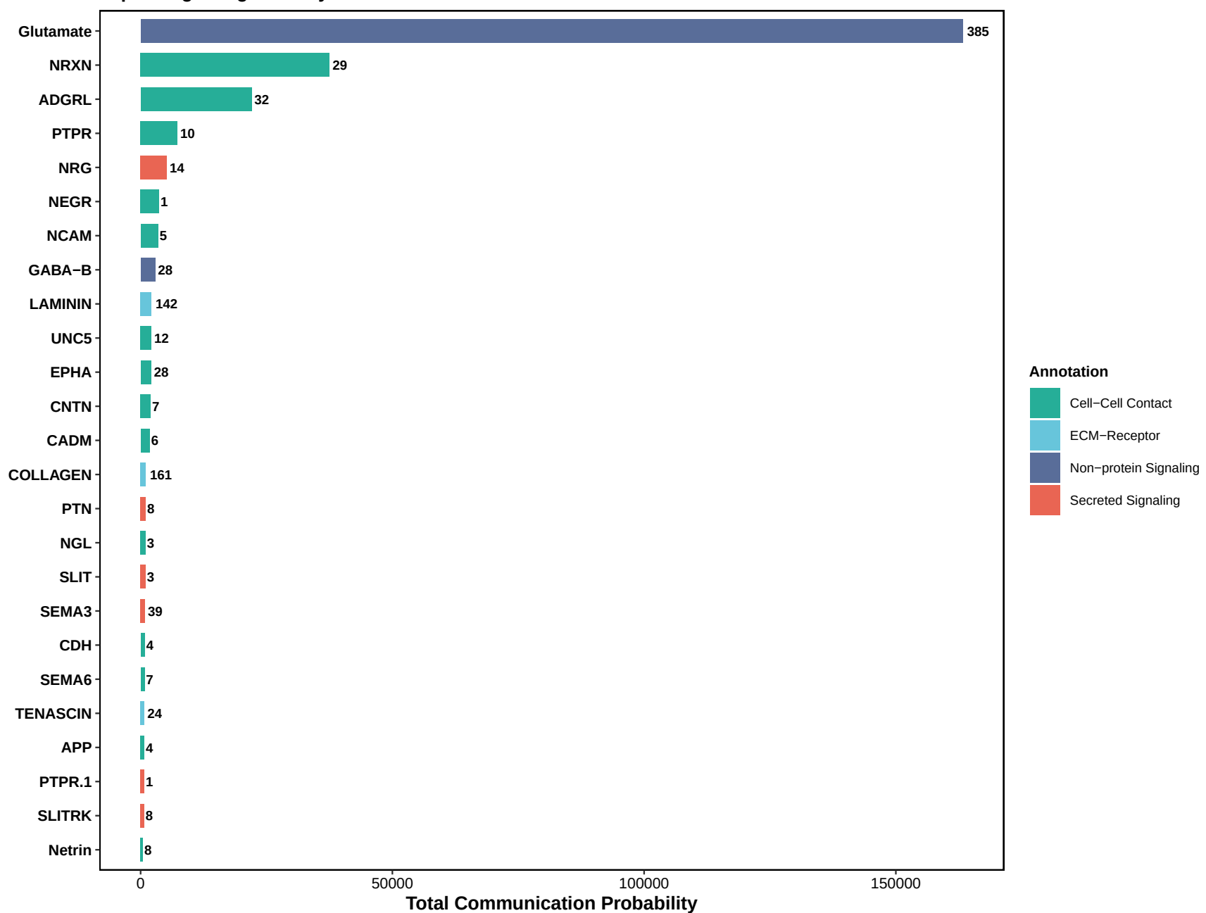
Top 25 Signaling Pathways
