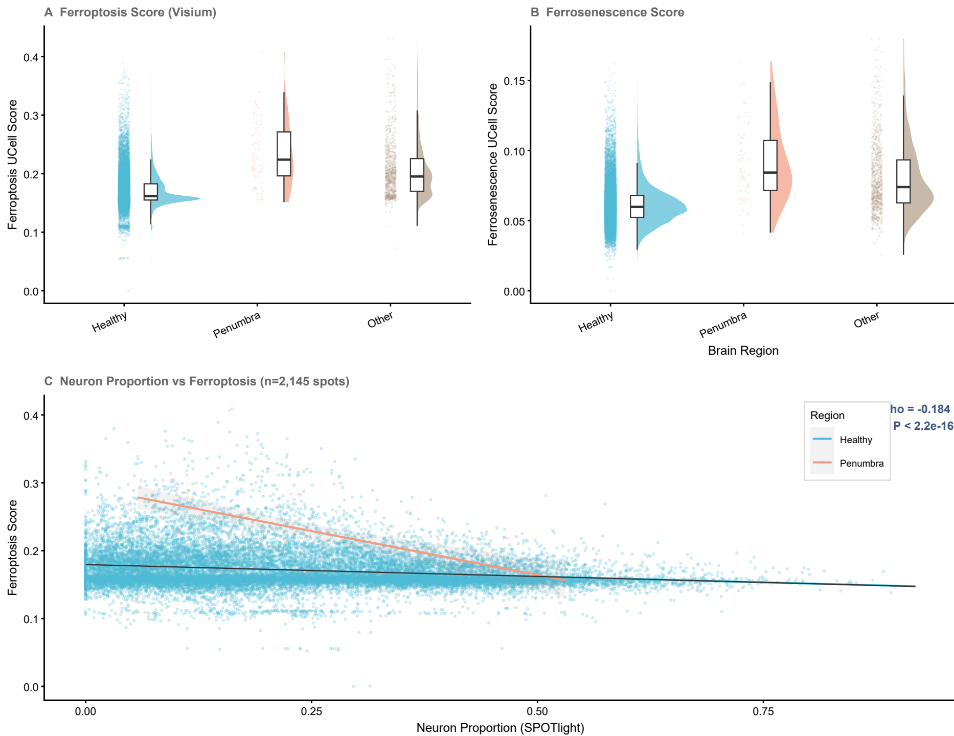
Figure 4: Spatial Localization of Iron-Aging Signals in CIRI Penumbra
