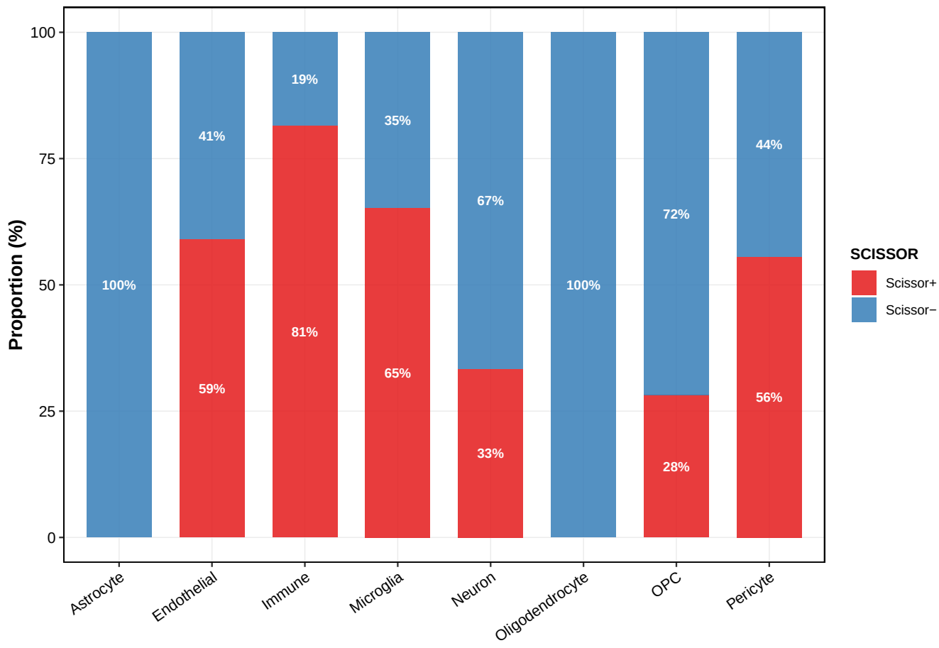
SCISSOR+/- proportion by cell type
