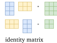
Figure 2.5 Even if both matrix multiplications \mathbf{AB} and \mathbf{BA} are defined, the dimensions of the results can be different.
