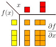
Figure 5.6 Dimensionality of (partial) derivatives.
