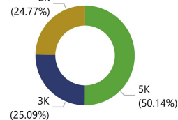
Customers and Churn Rate by Acct Balance
