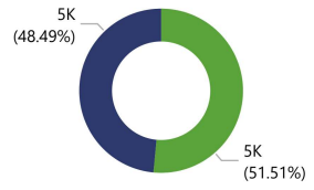
Customers and Churn Rate by Age Groups
