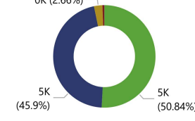
Customers and Churn Rate by Acct Balance
