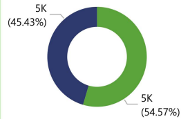
Customers and Churn Rate by Age Groups
