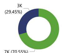
Customers and Churn Rate by Credit Scores
