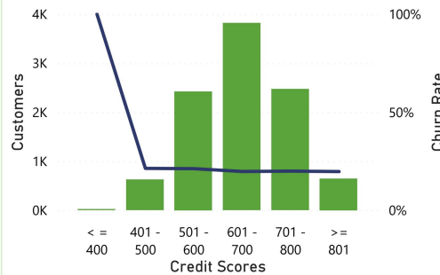
Customers and Churn Rate by Credit Scores
