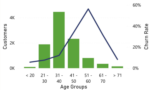
Customers and Churn Rate by Age Groups
