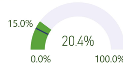
Customers by Country
