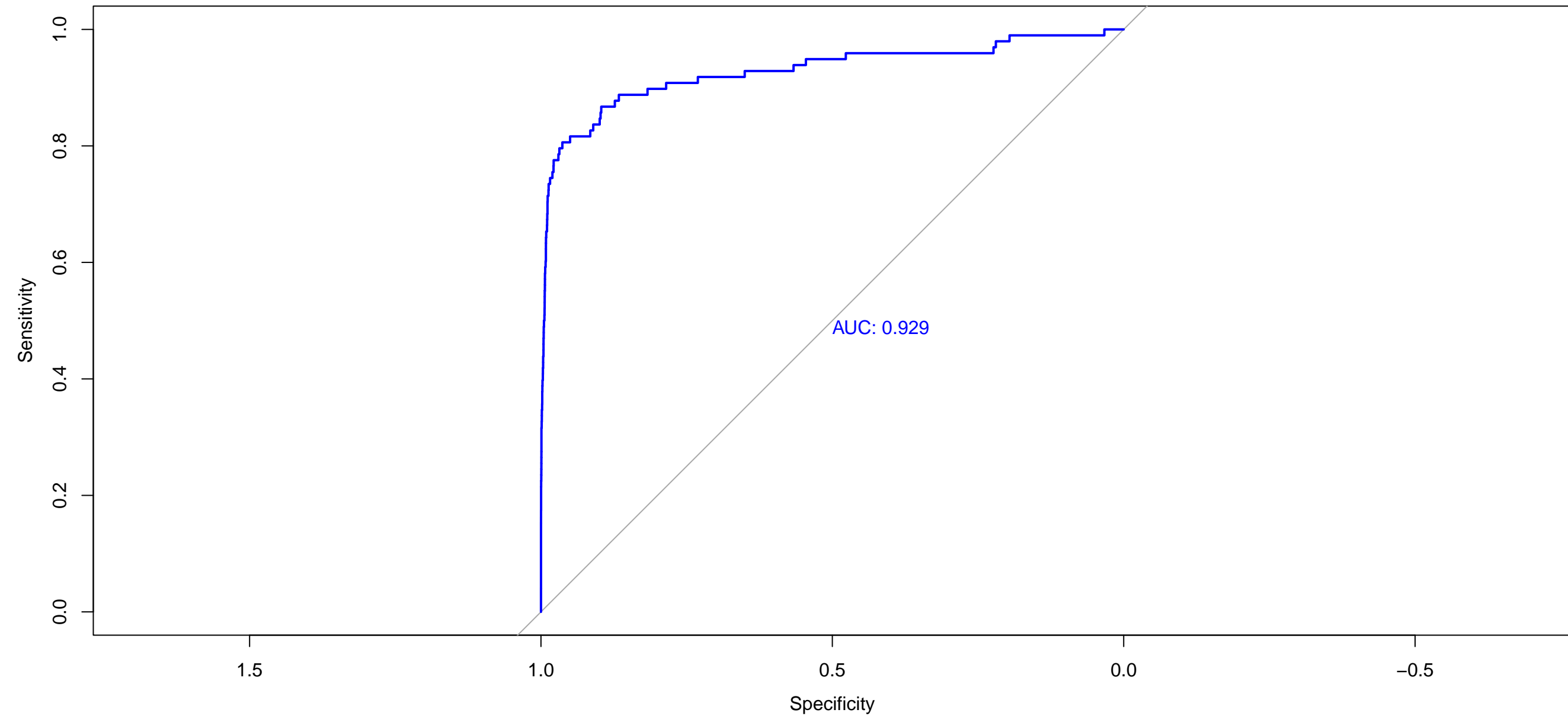
ROC Curve – Logistic Regression
