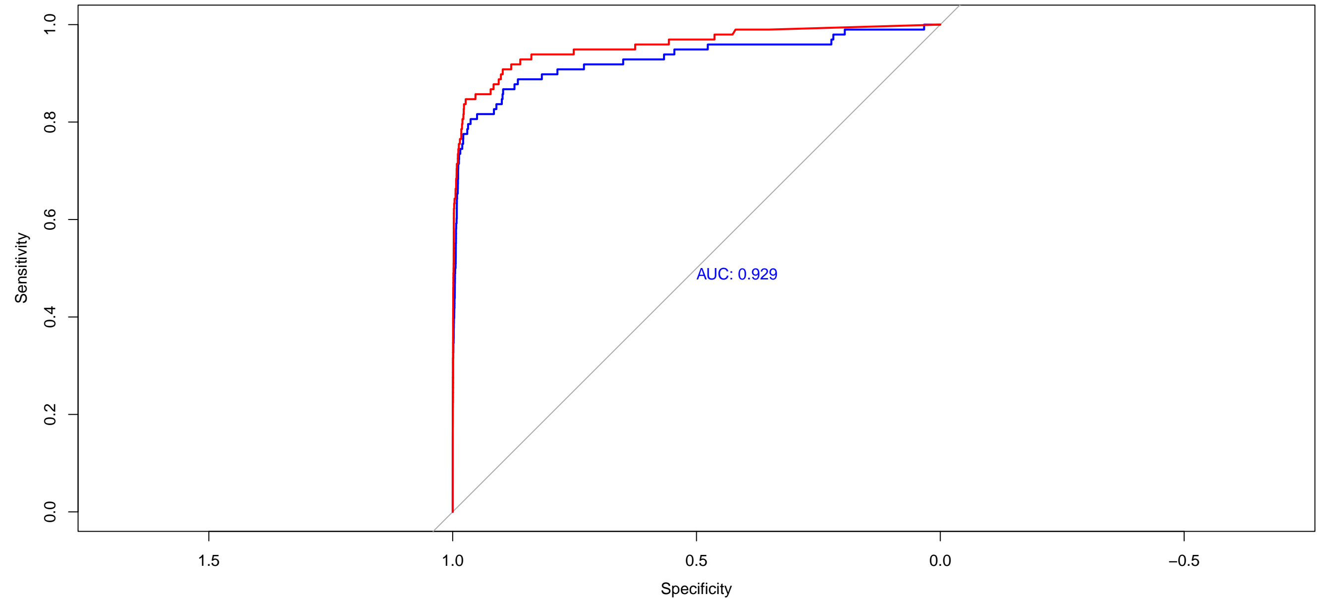
ROC Curve
