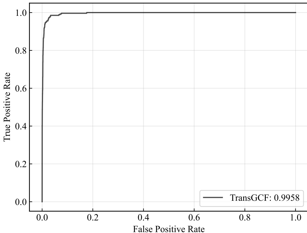
ROC Curve - abu-urban-4
