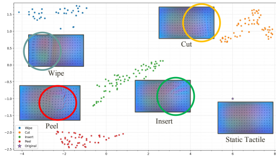
Figure 6: t-SNE visualization of tactile representations encoded by the pretrained Wan VAE. Different manipulation actions form distinct clusters in the latent space, and a representative tactile image is shown next to each cluster for reference.
