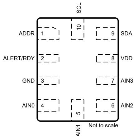
Figure 4-1. RUG Package, 10-Pin (Top View)
