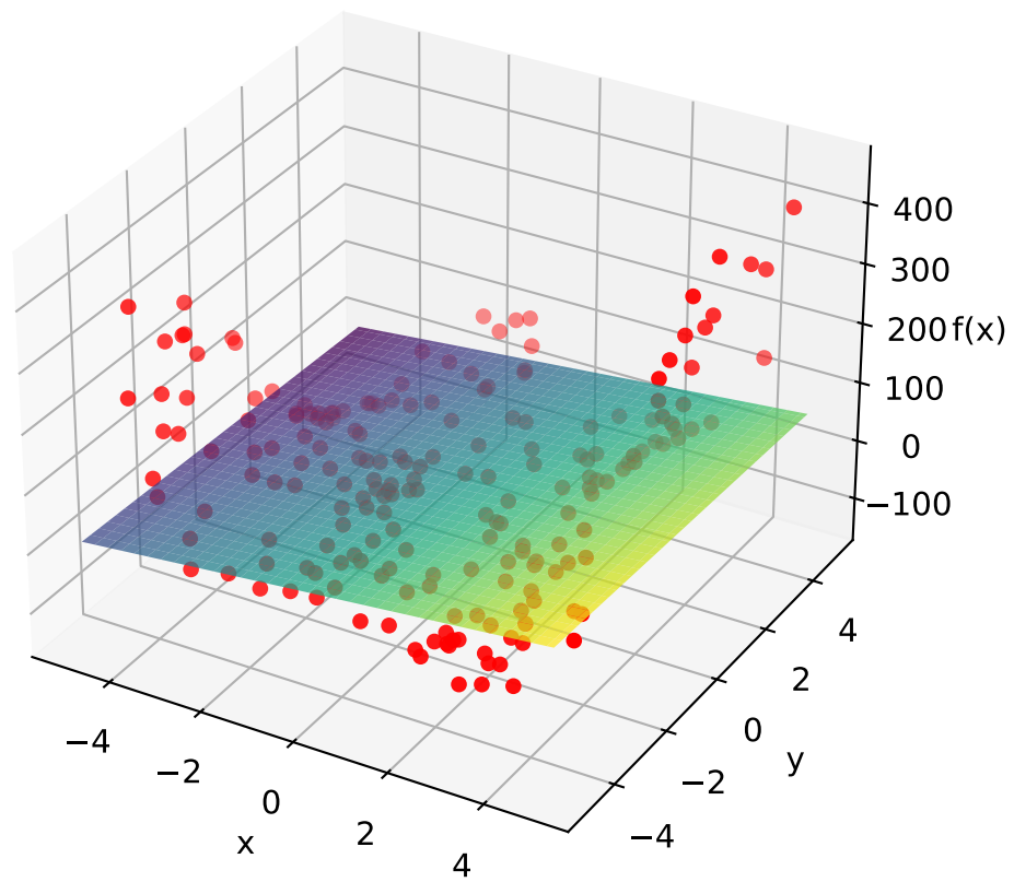
3 affine product
