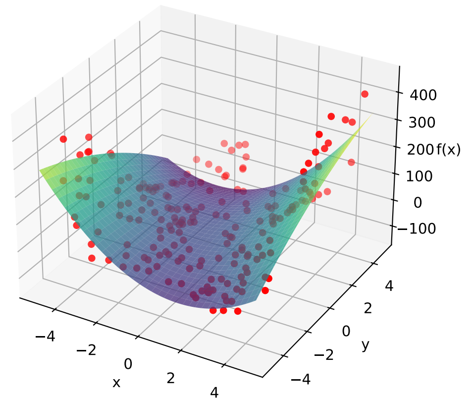
4 affine product
