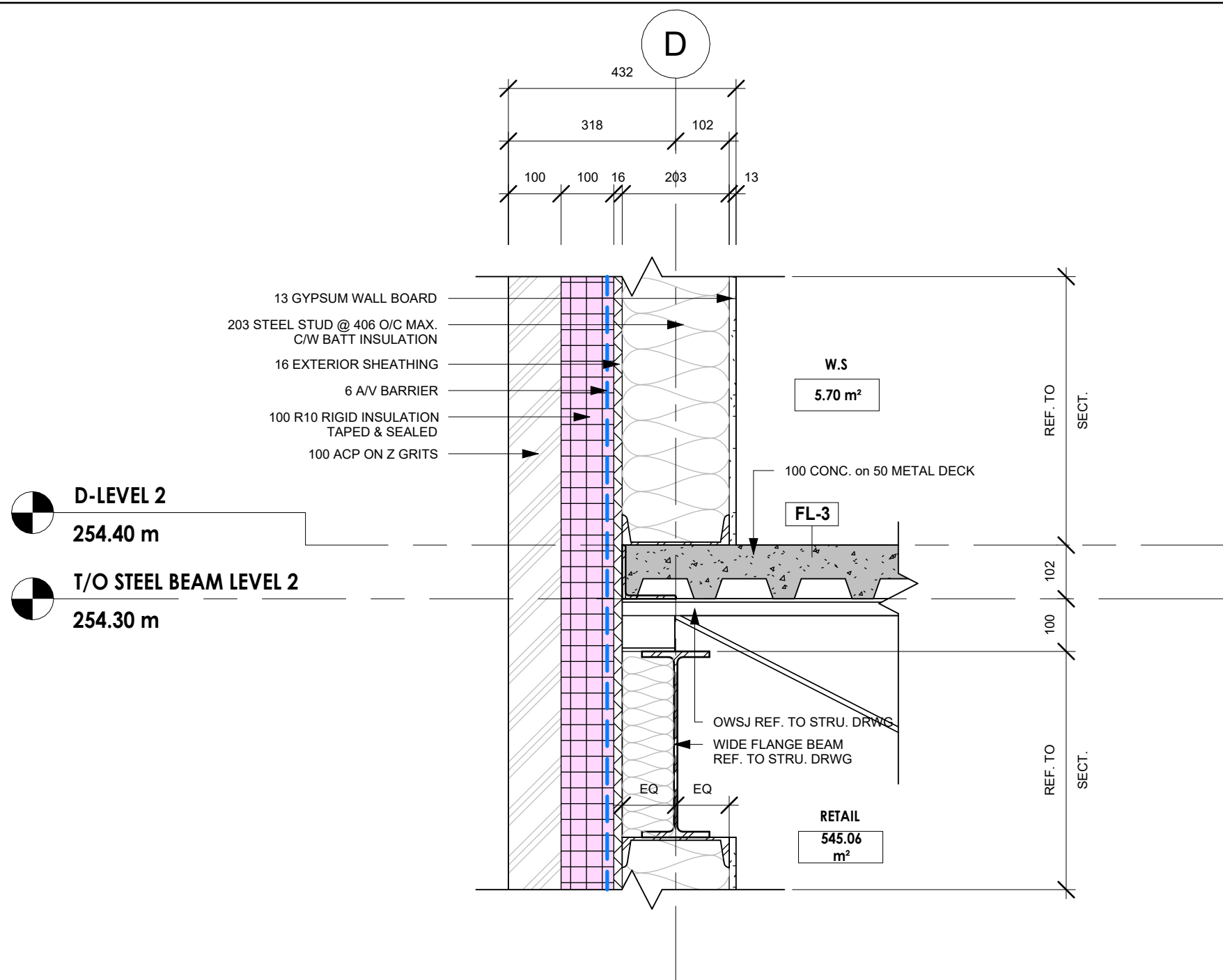
TYP. WALL TO FLOOR CONN. 1 : 10
