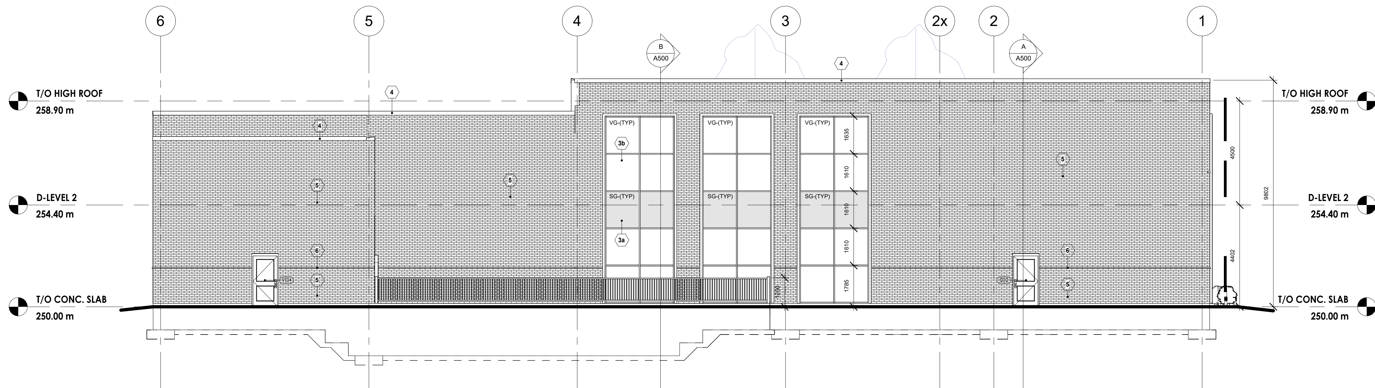
2 NORTH ELEVATION 1 : 100
