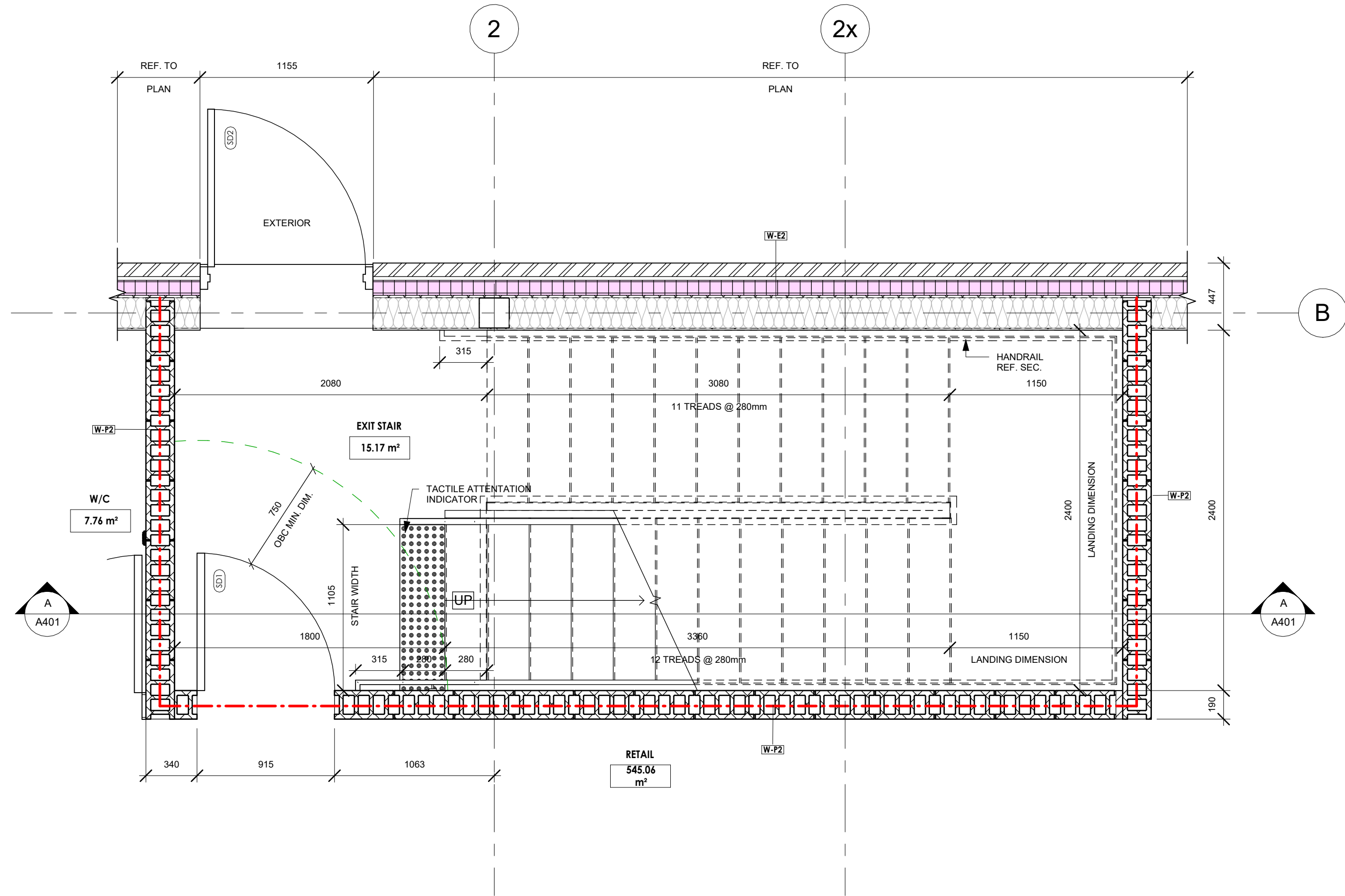
1 A400 ENLARGED MAIN FLOOR STAIR PLAN 1 : 25
