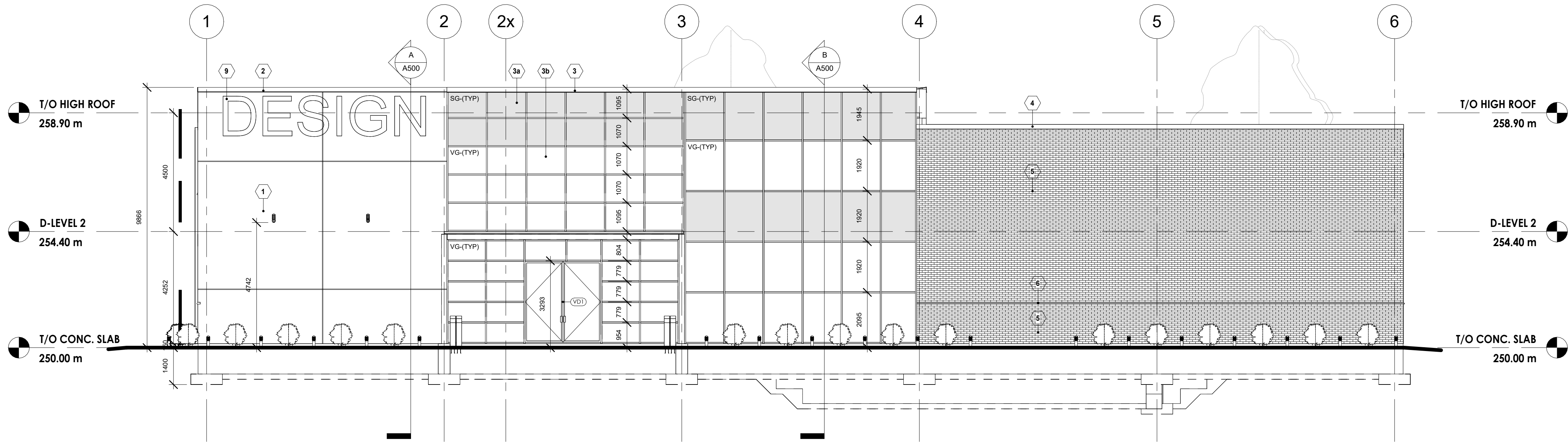
1 SOUTH ELEVATION 1 : 100
