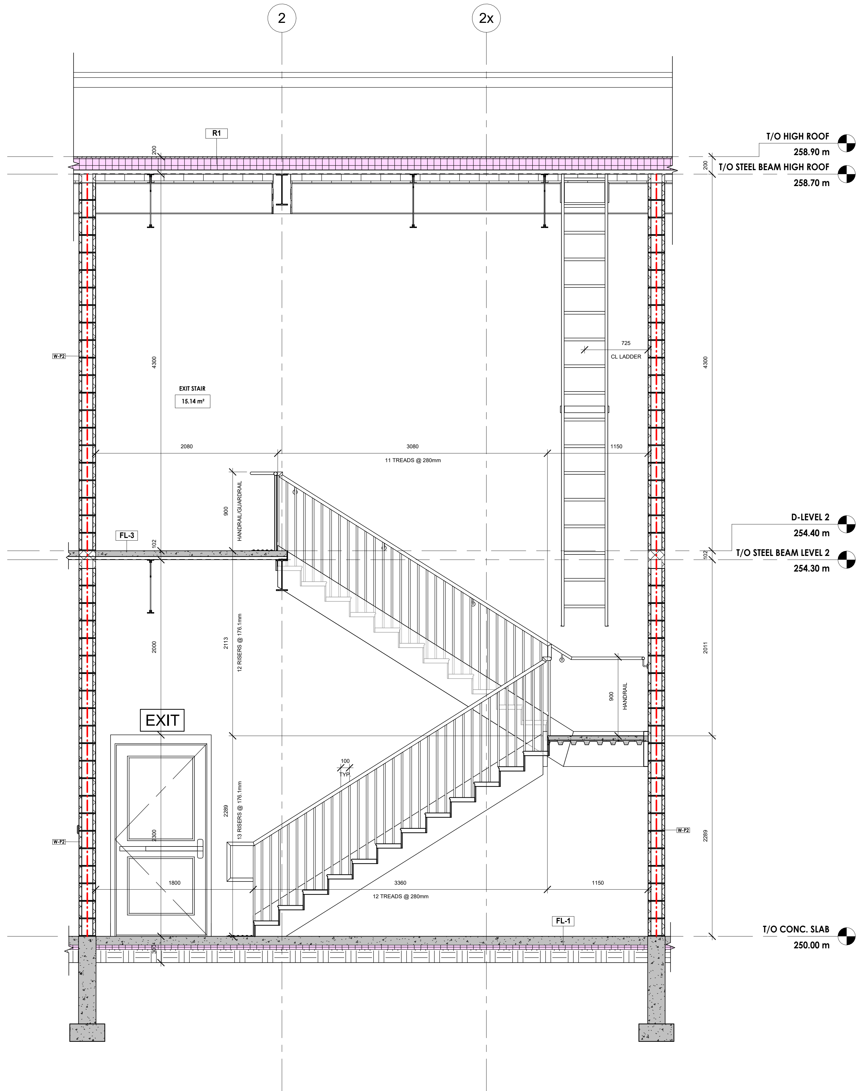
STAIR SECTION
