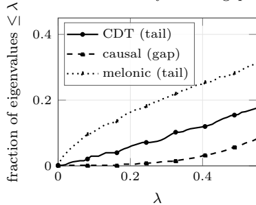
near-0 density: tail vs gap
