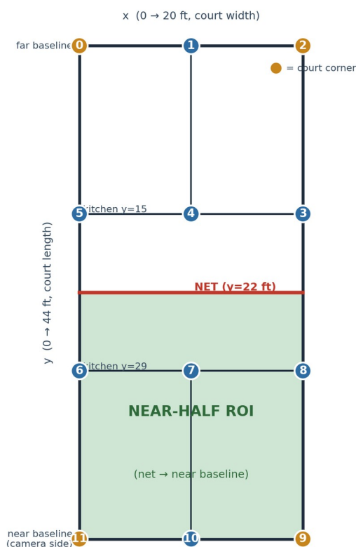
Canonical 12-keypoint court model (origin at far-baseline-left)
