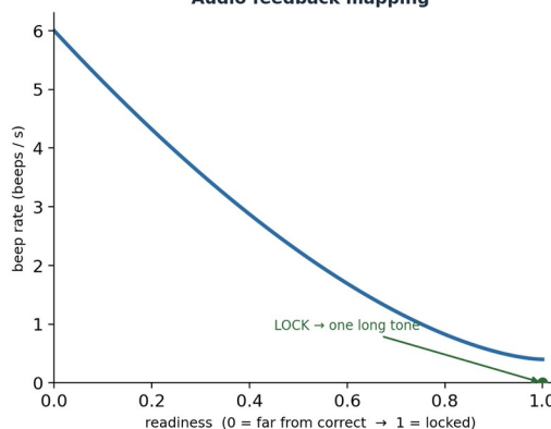
Figure 8. Guided-placement state machine and audio-feedback mapping. Searching (rapid beeps) → Aligning (beeps slow as readiness rises) → Locked (one long tone). The gate is all four corners visible plus a stable low-error homography.
