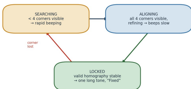
Placement-guidance state machine
