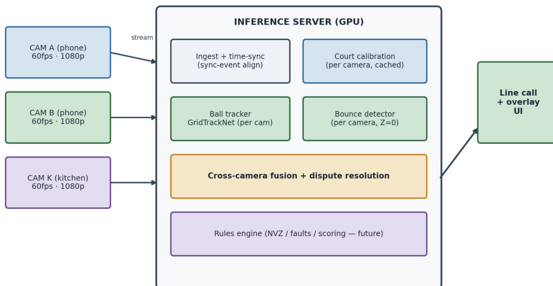
Proposed real-time architecture: phones stream to a GPU server that returns instantaneous calls
