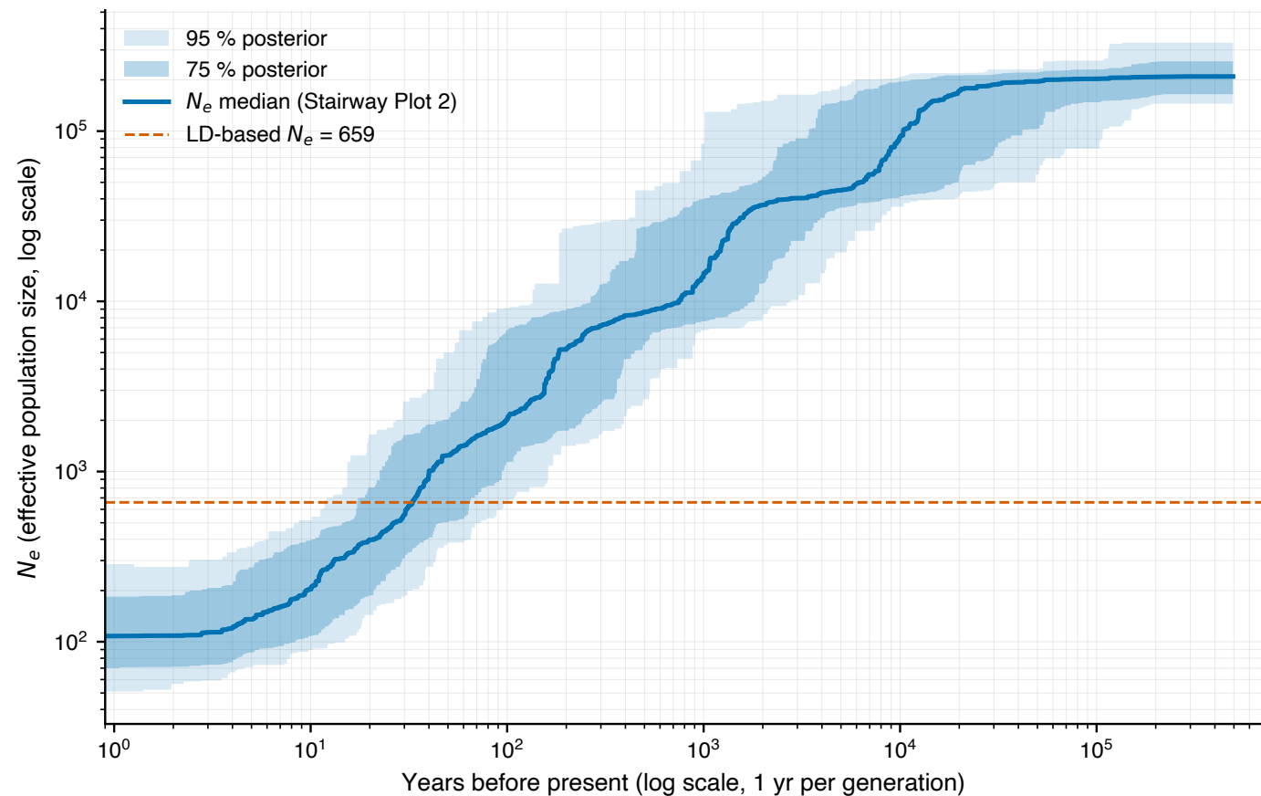
Stairway Plot 2 N_e(t) trajectory (African yam bean, n = 95 IITA TSs panel)
