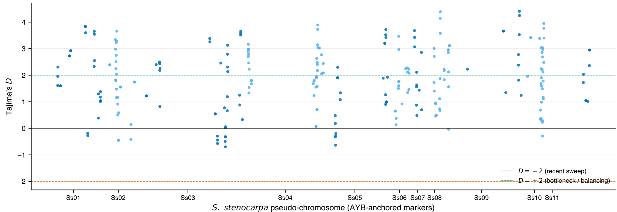
Windowed Tajima's D across the genome (255 windows, 250 kb / 100 kb)
