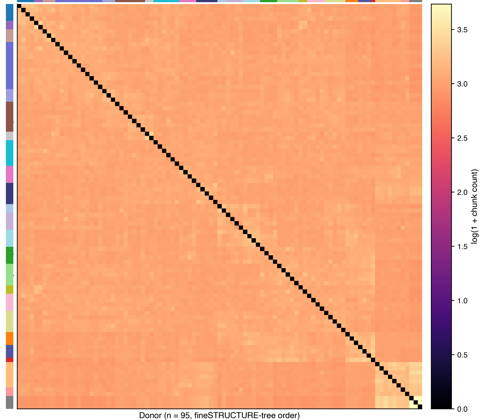
ChromoPainter coancestry, MAP K = 24 (African yam bean 95-line panel)
