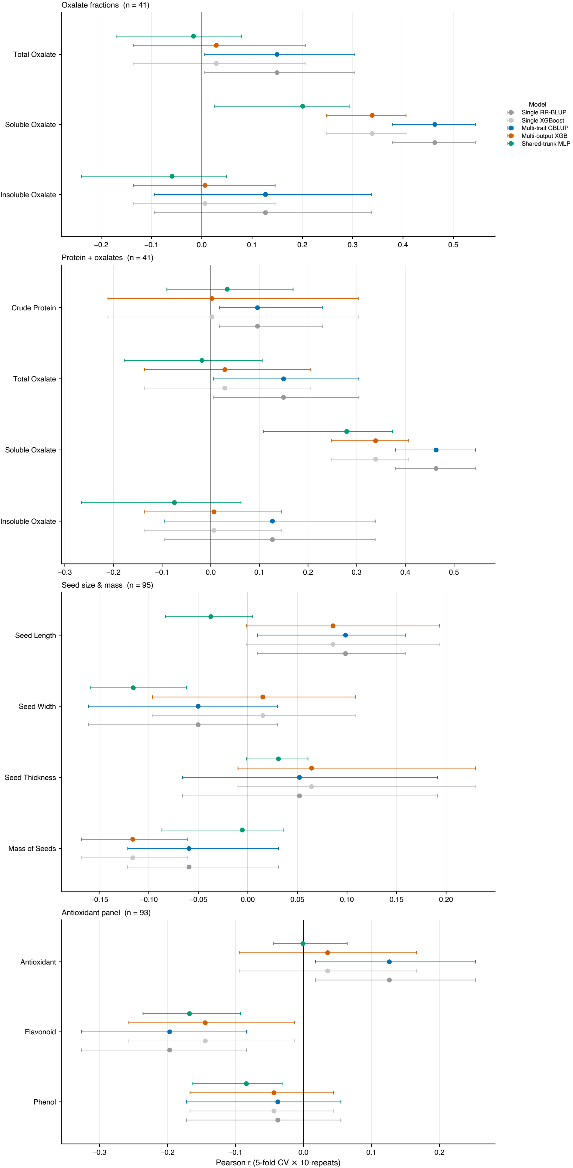
Multi-task vs single-trait genomic prediction (AYB DArTseq panel)
