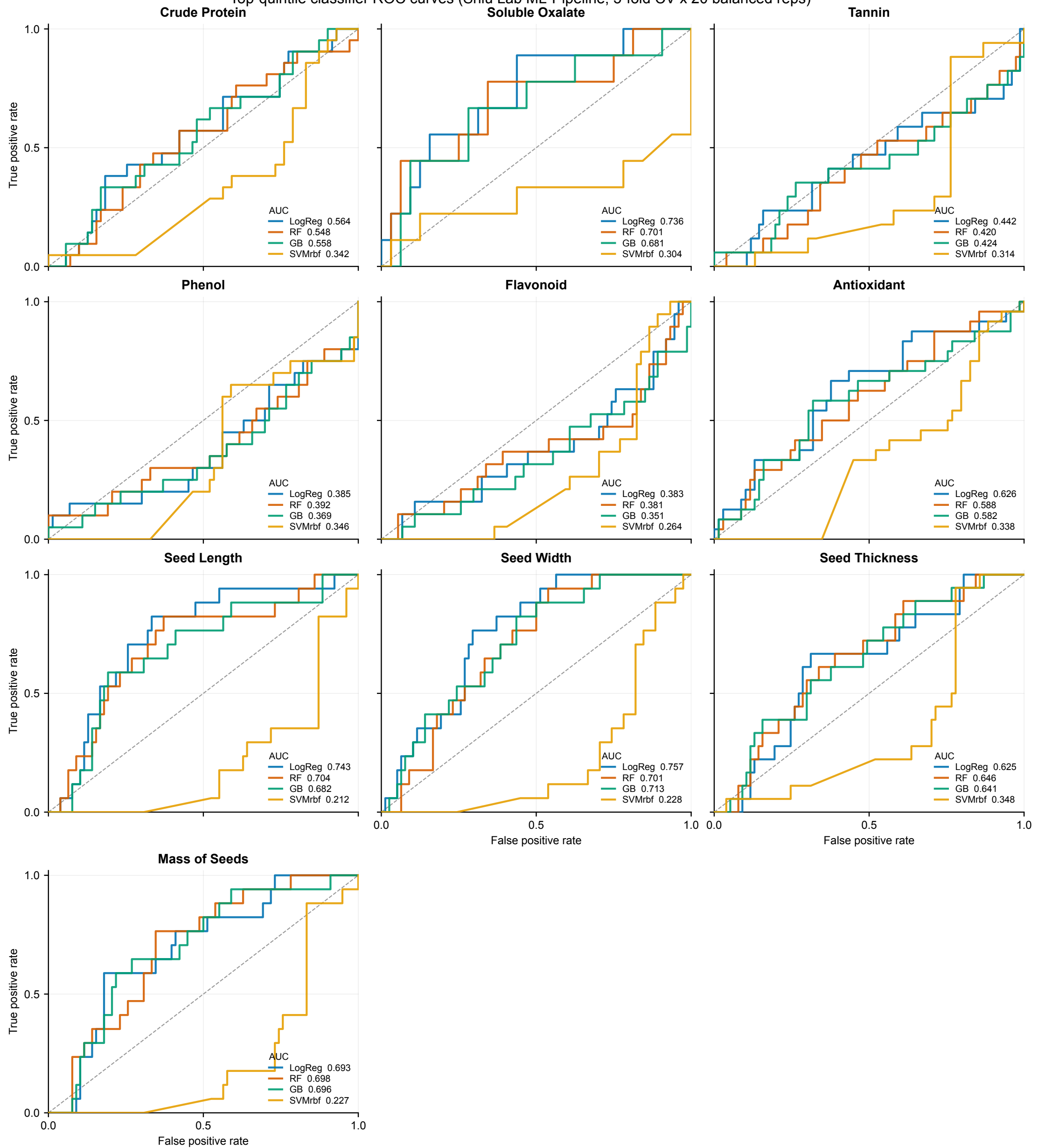
Top-quintile classifier ROC curves (Shiu Lab ML-Pipeline, 5-fold CV x 20 balanced reps)
