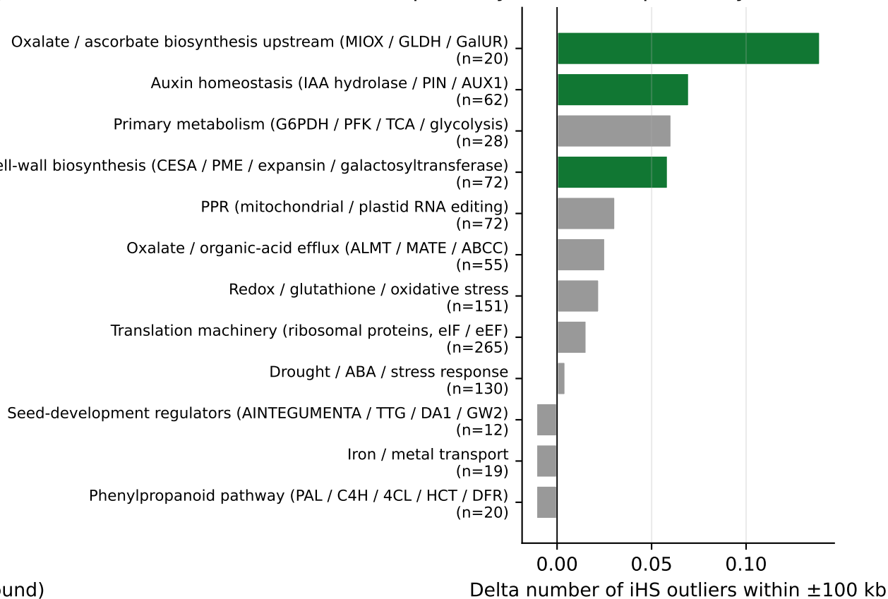
b Per-pathway iHS-outlier-proximity delta vs background
