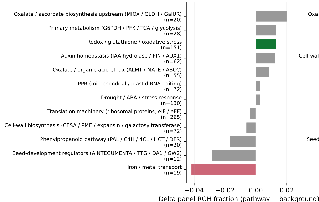
a Per-pathway ROH-density delta vs background
