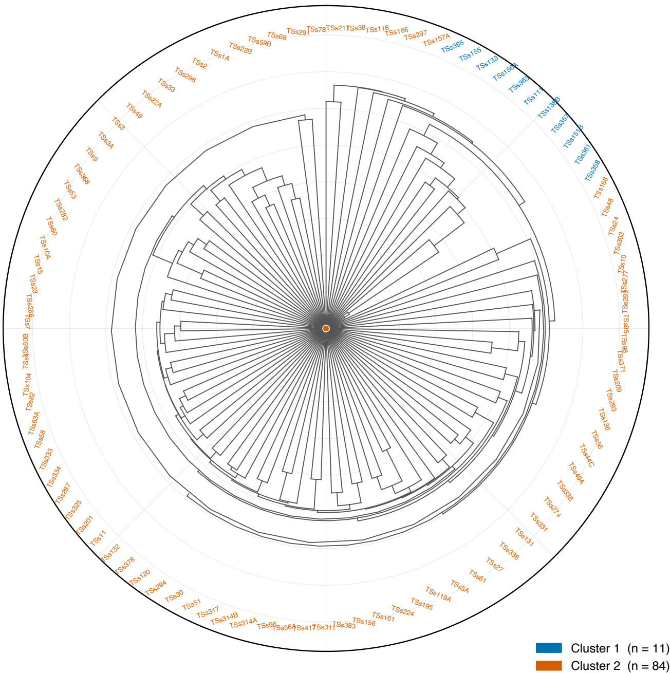
Circular UPGMA dendrogram — 95 AYB lines, 1,625 QC SNPs
