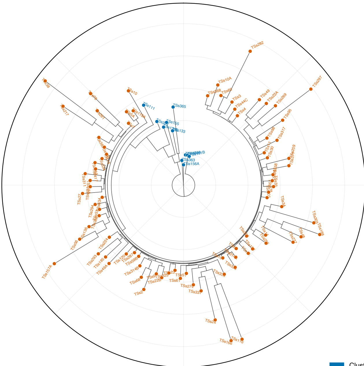
IQ-TREE (GTR+ASC, UFBoot1000) — 95 AYB lines
