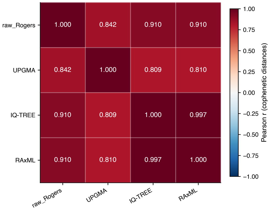
Cophenetic distance correlation across tree methods
