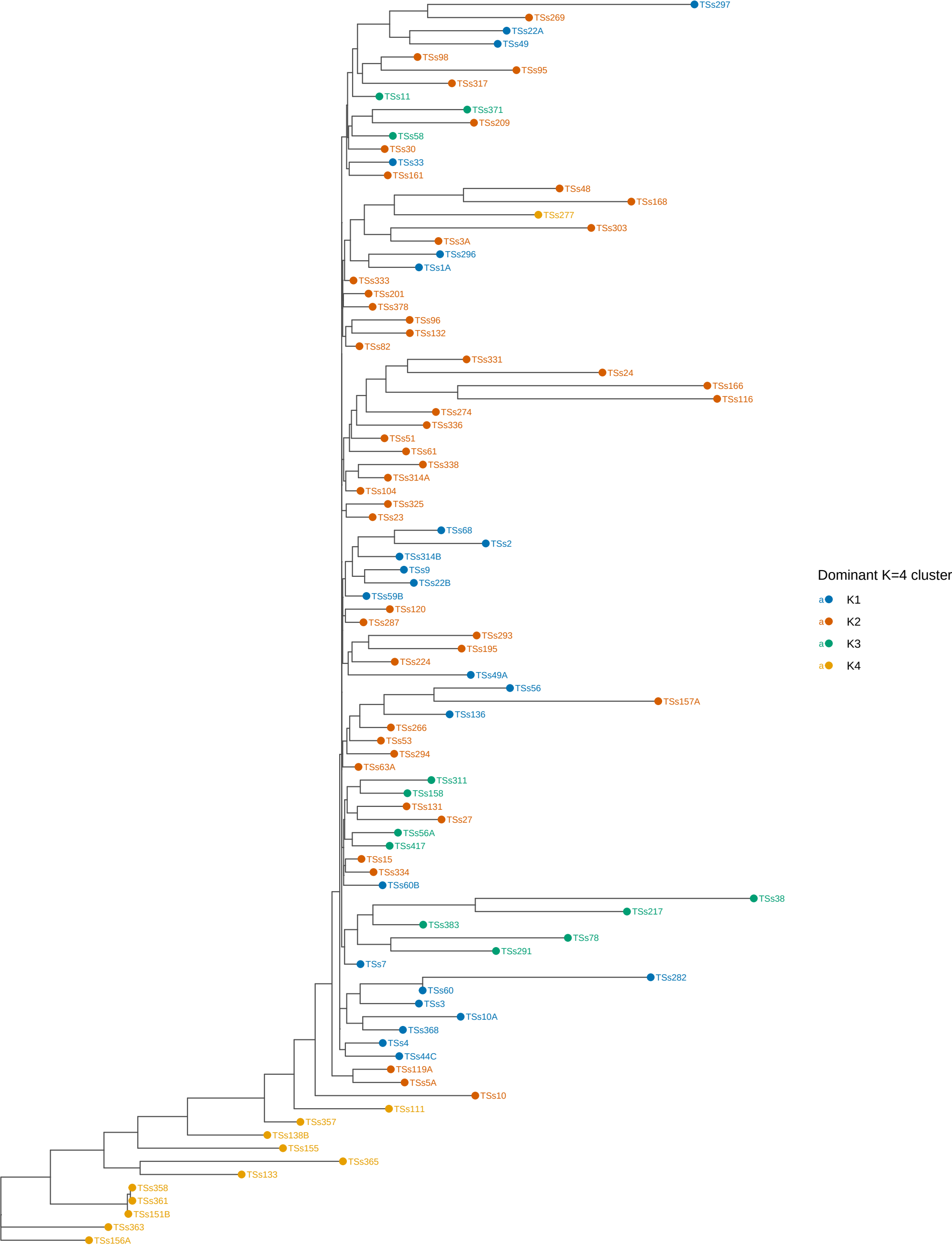
IQ-TREE 3.0.1 ML phylogeny with tips coloured by dominant ADMIXTURE K=4 cluster
