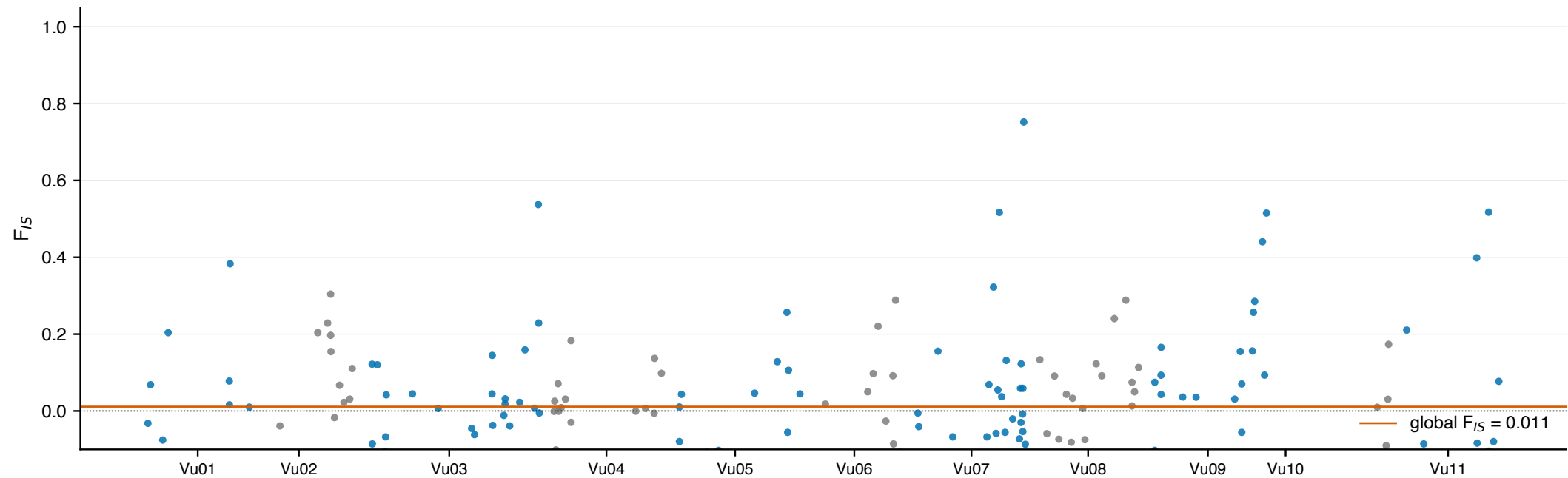
Per-locus F_{IS} across cowpea-anchored 175 SNPs
