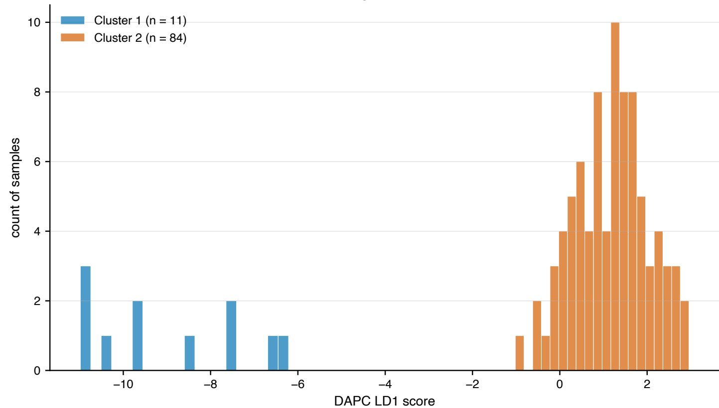
DAPC LD1 separating marker-PCA k = 2 clusters
