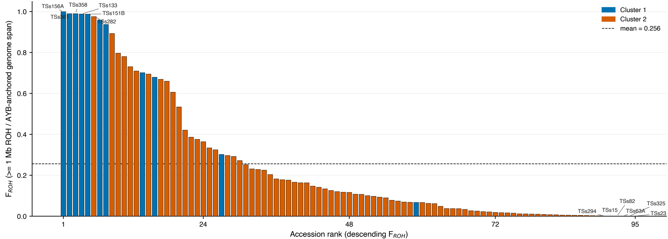
Per-accession F_{ROH} ( \geq 1 Mb segments) -- selfer-paper individual-inbreeding measure (95 accessions)
