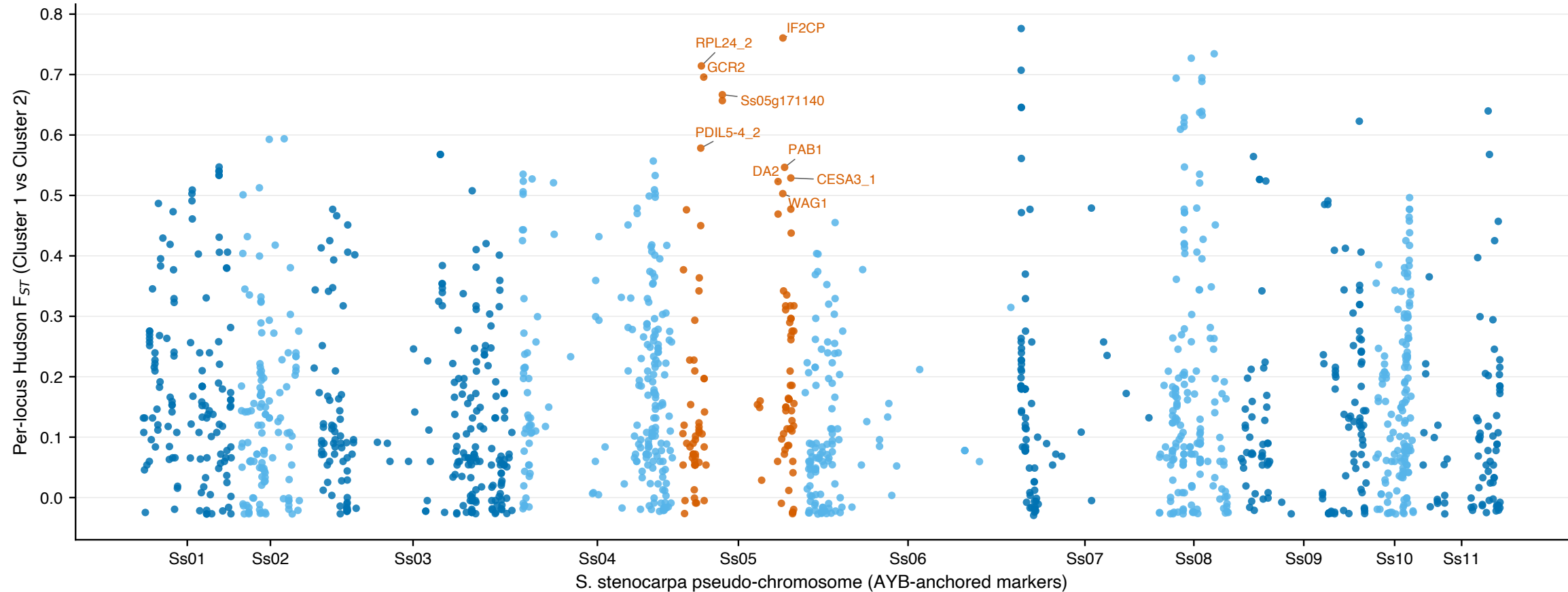
Per-locus Hudson F_{ST} across AYB-anchored markers; Ss05 highlighted with top-10 nearest-gene callouts
