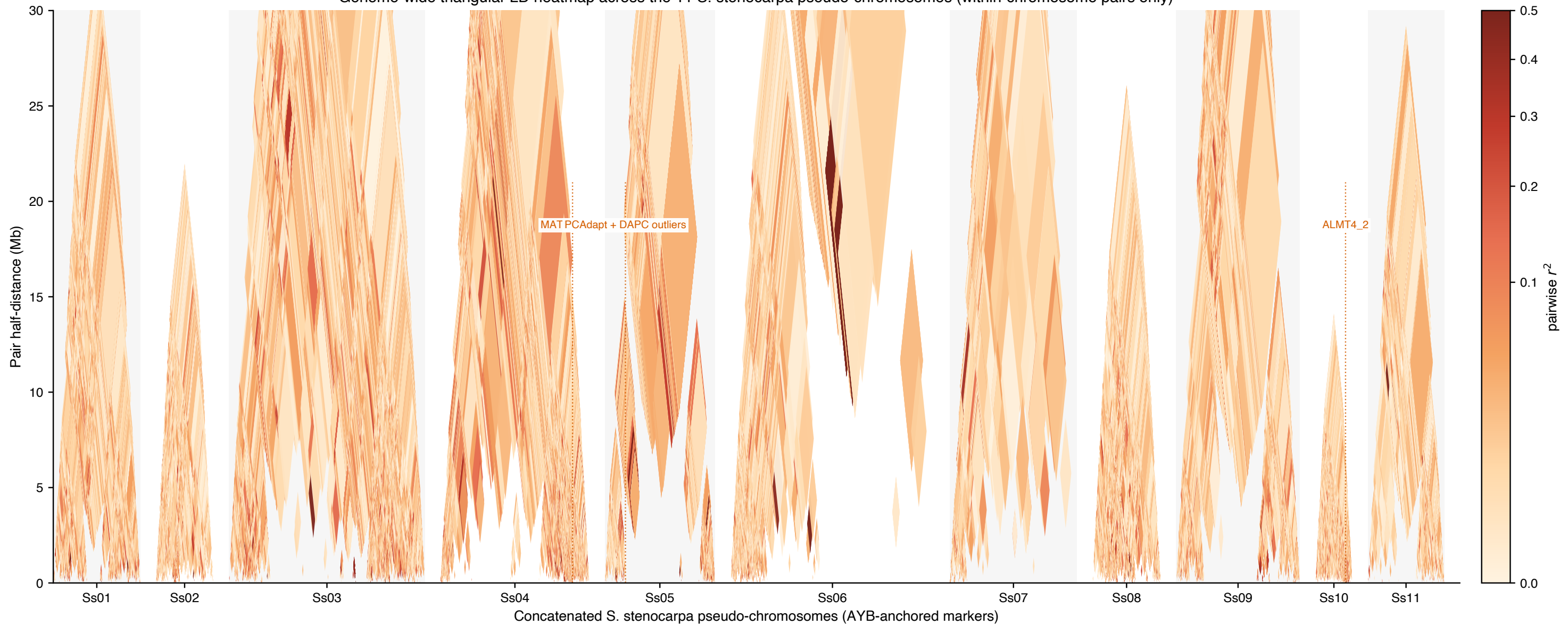
Genome-wide triangular LD heatmap across the 11 S. stenocarpa pseudo-chromosomes (within-chromosome pairs only)
