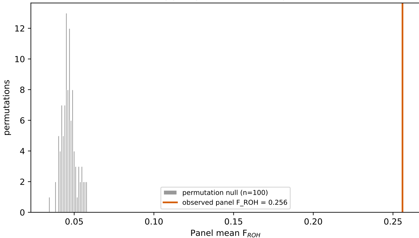
Observed autozygosity vs within-locus permutation null
