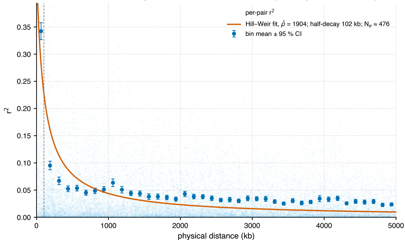
Genome-wide LD decay across AYB-anchored markers (32,507 pairs, Ss01–Ss11)
