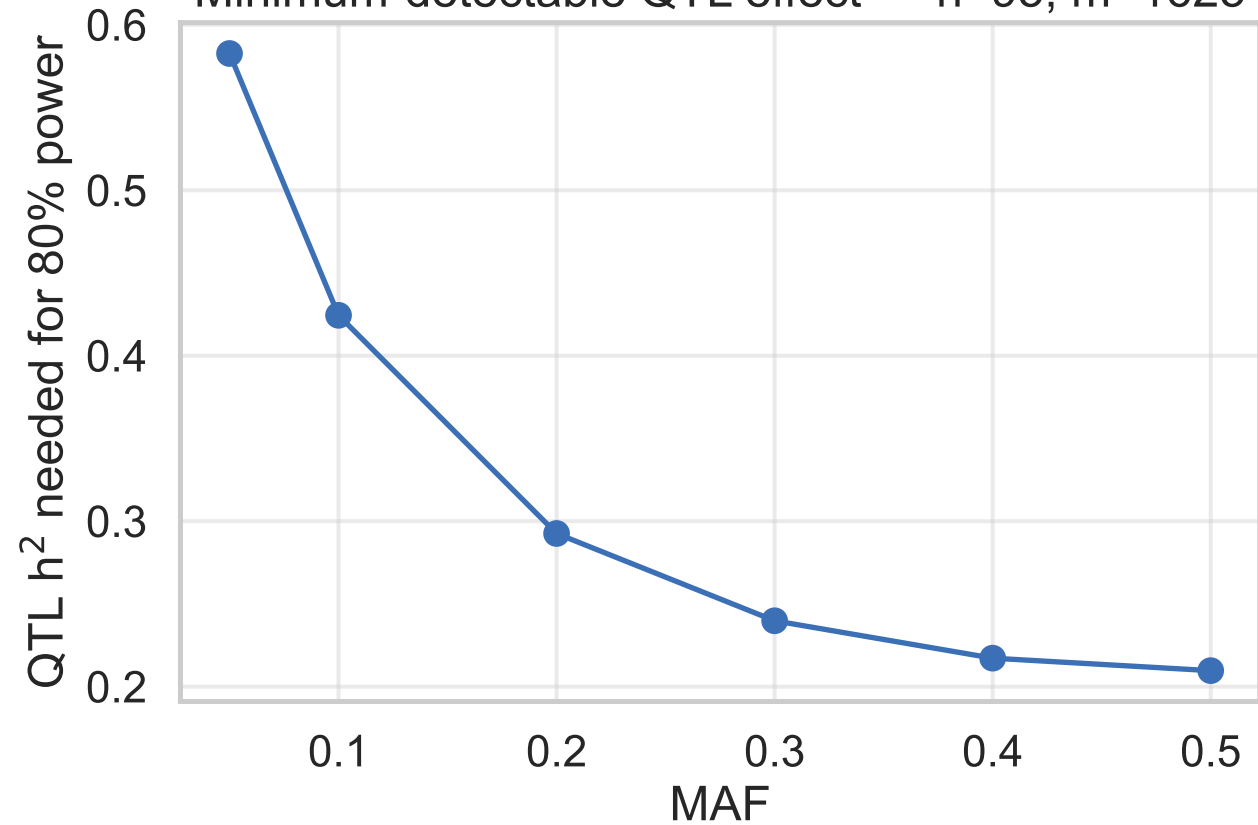
Minimum-detectable QTL effect — n=95 , m=1625
