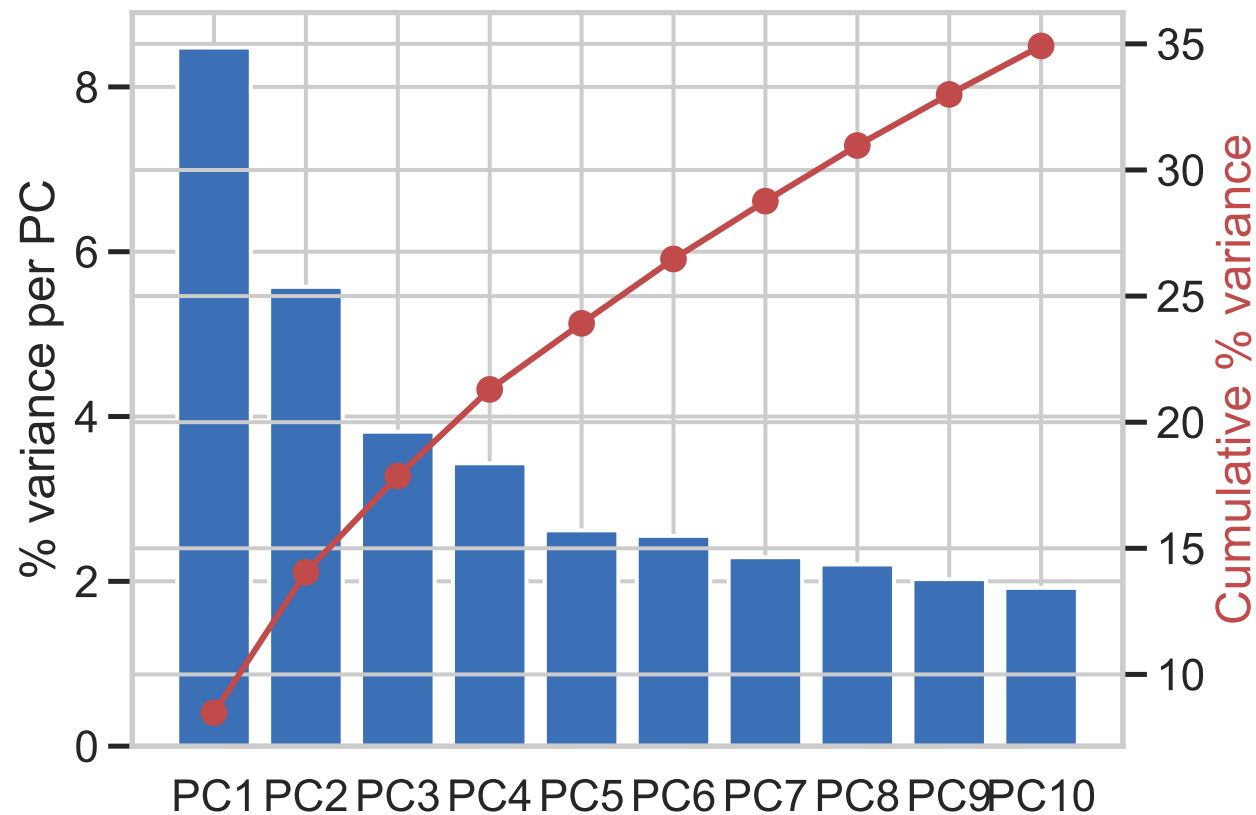
PCA scree — 1625 SNPs after QC
